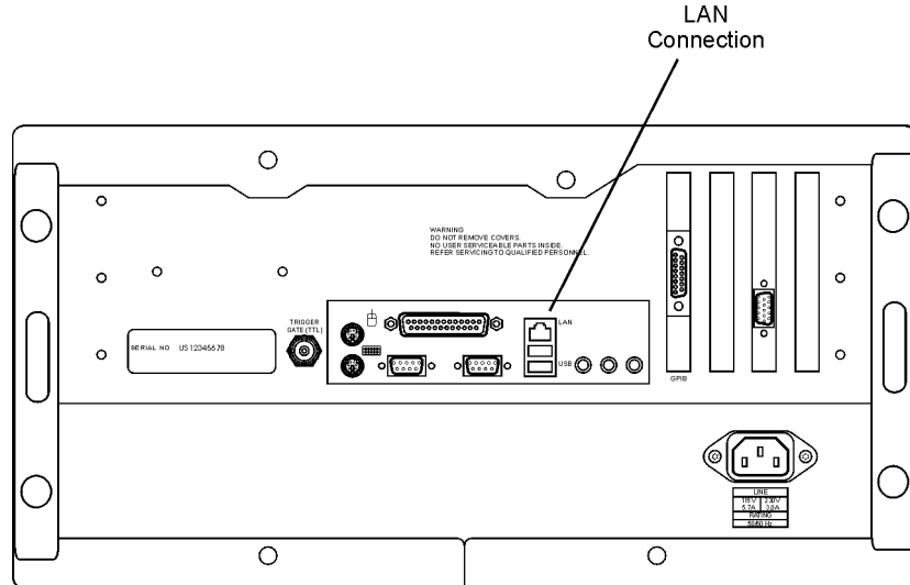
Figure 1-21. LAN Connector
